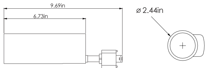
TL02-20W
